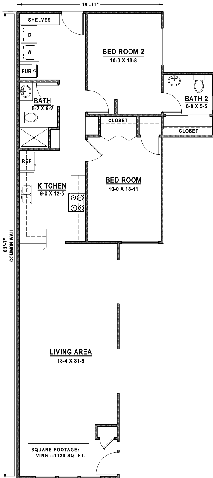
AC 2: 2-BEDROOM SCALE 1/8" = 1'0"
