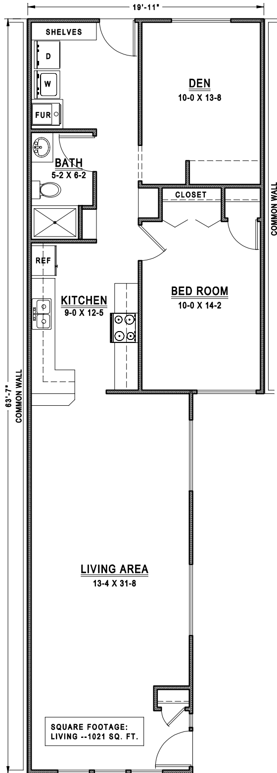
AC 2: 1-BEDROOM/DEN SCALE 1/8" = 1'0"
